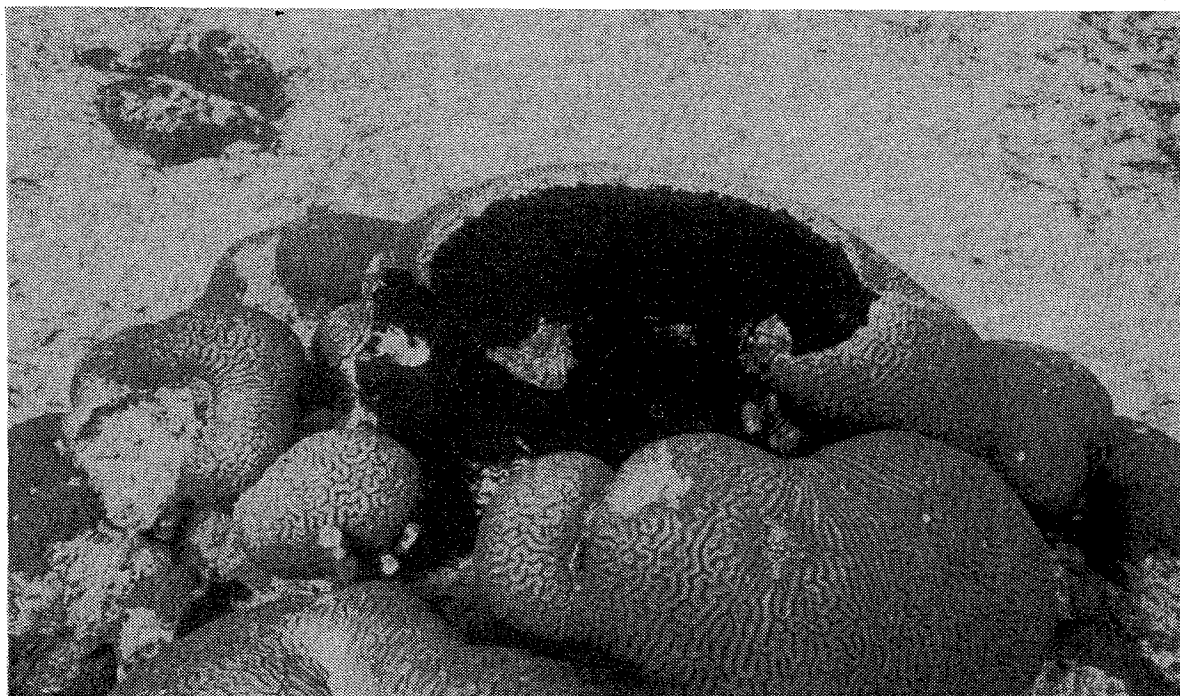
Fig. 7. The hadromerid sponge Cliona caribbea growing on a large Diploria labyrinthiformis . It probably started out at some spot of denuded coral skeleton, but proceeds to overgrow living coral surface.
