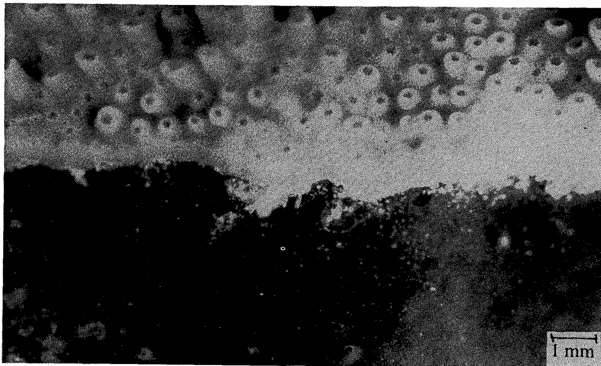
Fig. 8. Close-up of the advancing front of Cliona caribbea on an Acropora palmata . The sponge not only kills off the coral polyps, but also penetrates the uppermost layer of the skeleton.
