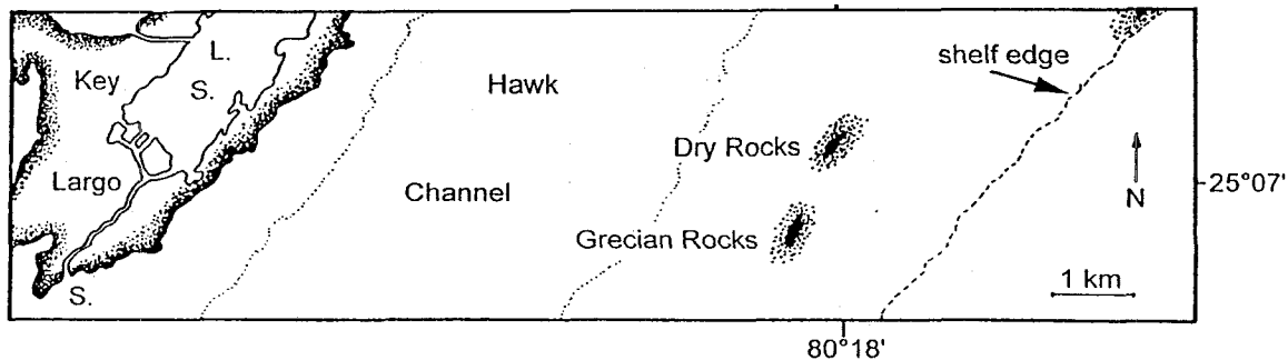
Fig. 2. To the left (= west) Key Largo with Largo Sound (L. S.) and South Sound Creek (S.). To the right (= east) the White Banks area with the Key Largo Dry Rocks and Grecian Rocks reefs. The shelf edge marks the 30m isobath.
