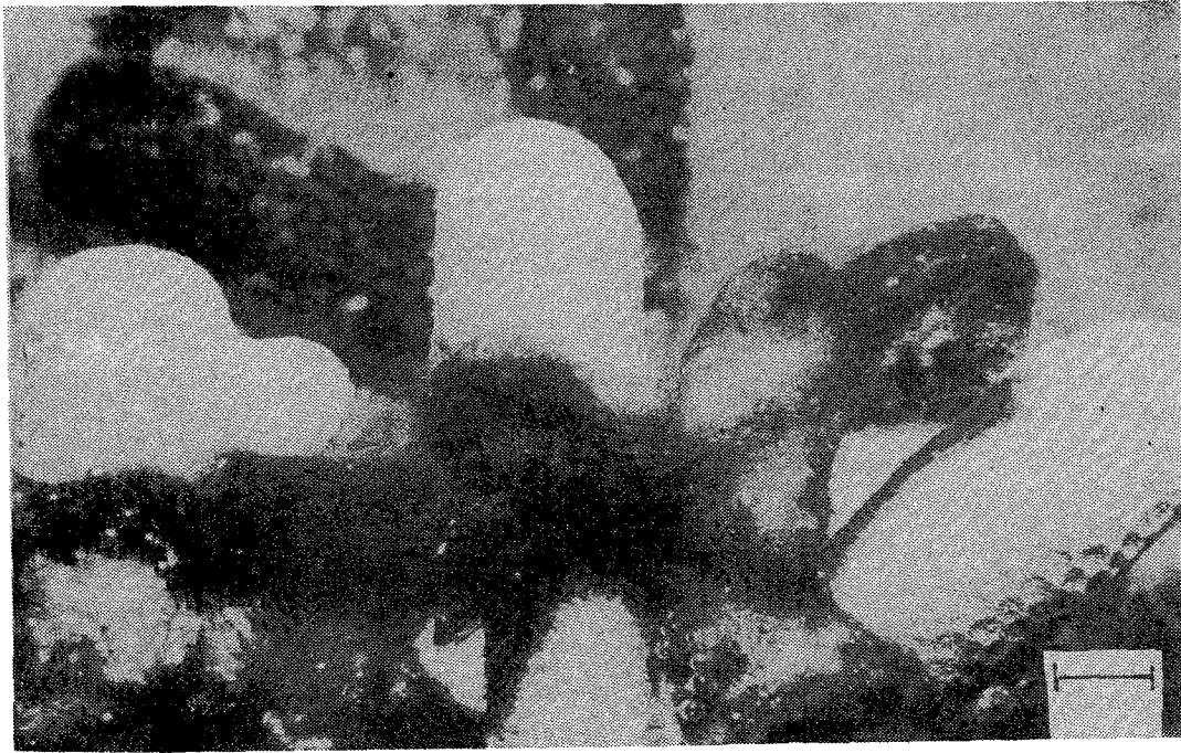
Fig. 3. The typical "tufts" of Oscillatoria submembranacea on branches of Porites porites . One of the branches has been completely covered by the cyanophyte.
