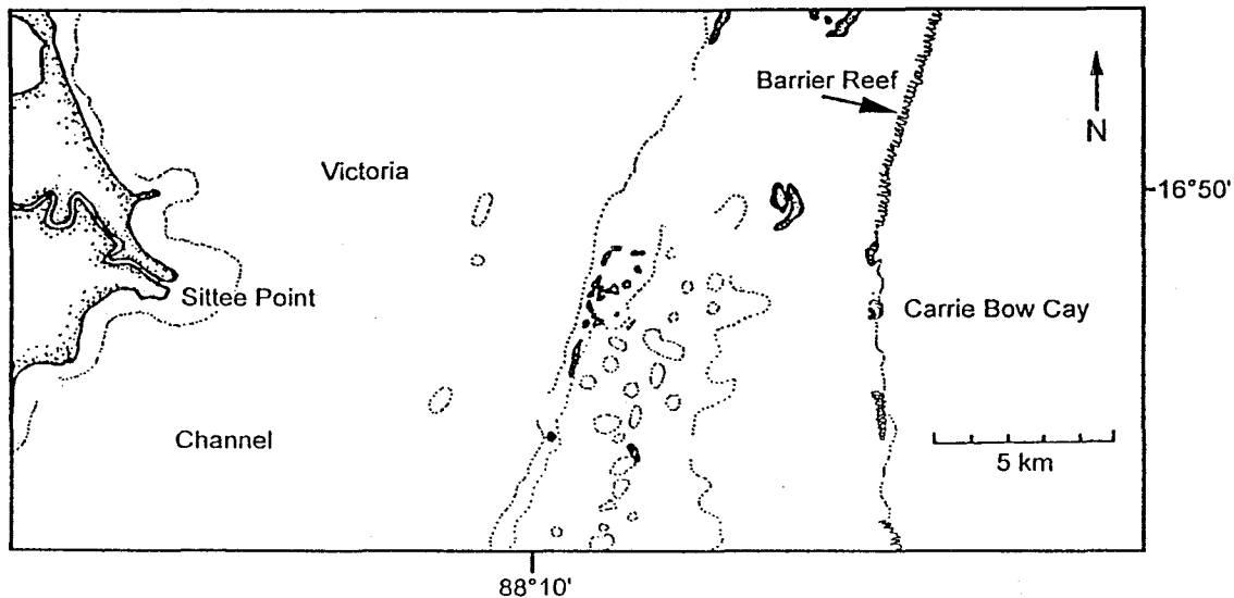
Fig. 1. To the left (= west) the mainland of Belize just south of the town of Dangriga with the mouth of the Sittee River. To the right (= east) the patch-reef system of the lagoon and the barrier reef with Tobacco Reef in the north, Curlew Bank in the south and Carrie Bow Cay in the center.
