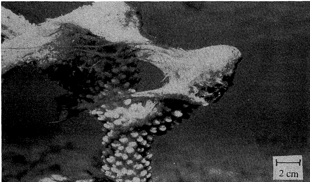
Fig. 4. Waving "flags" of Schizothrix mexicana on branch-tips of Acropora cervicornis . Coral tissue is being killed by the cyanophytic cover.
