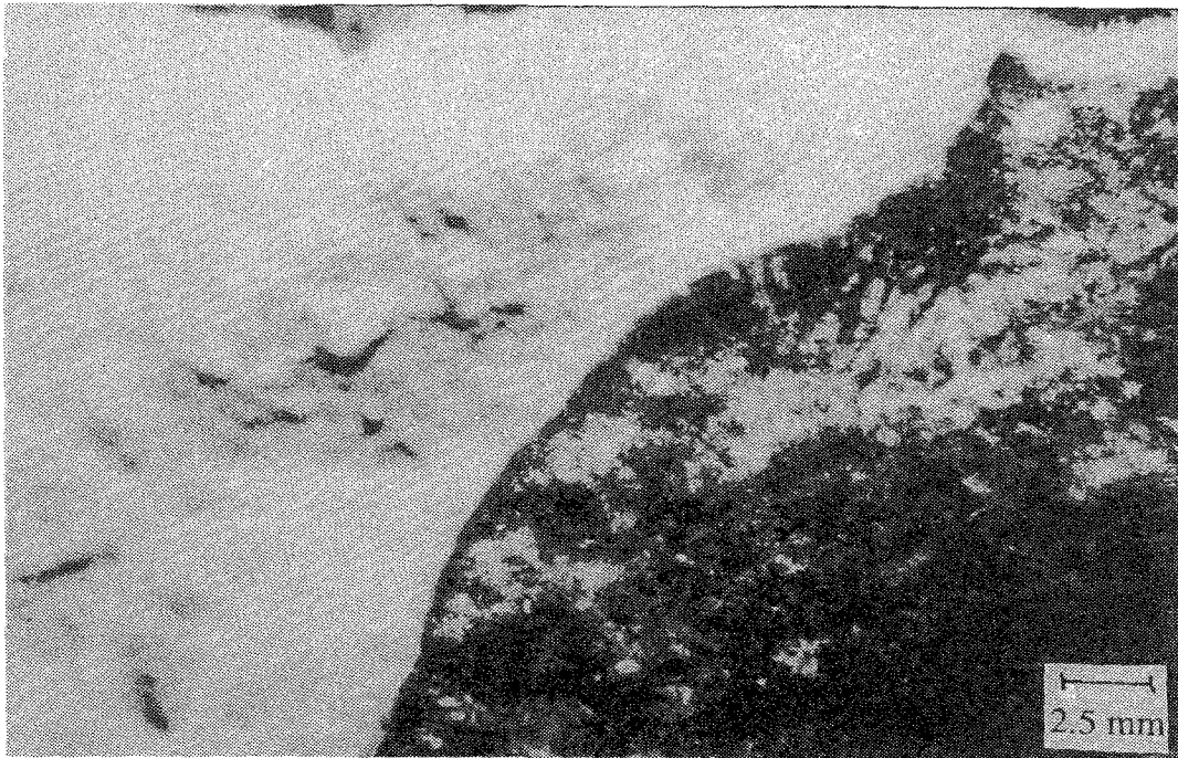
Fig. 5. The rhodophyte Metapeyssonnella corallepida growing over Millepora complanata . The edge of the alga is relatively straight and its color is a dark purple.
