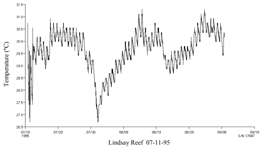
Fig. 4b. Electronic temperature data logger from Lindsay's Reef at 3 m depth from July through November 1995.
