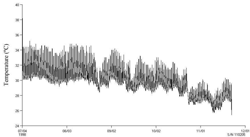
Fig. 5. Electronic temperature data logger from Lindsay's Reef at 3 m depth from July through November 1998.
