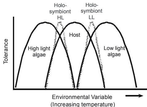
Fig. 6. Proposed model to explain the patterns of bleaching as a result of the different thermal tolerance limits of the holo-symbiont, the host and the high light (HL) and low light (LL) algal populations.
