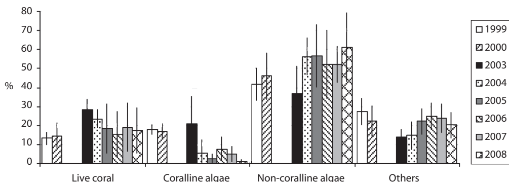
Fig. 8. Reef substrate relative cover at Meager Shoal (PNC), from 1999 to 2008.
