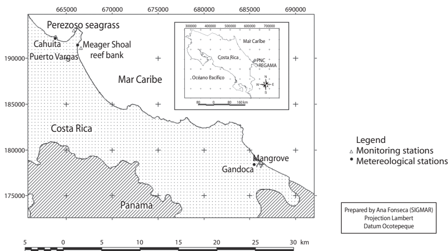
Fig. 1. Map of CARICOMP sites in Costa Rica.
