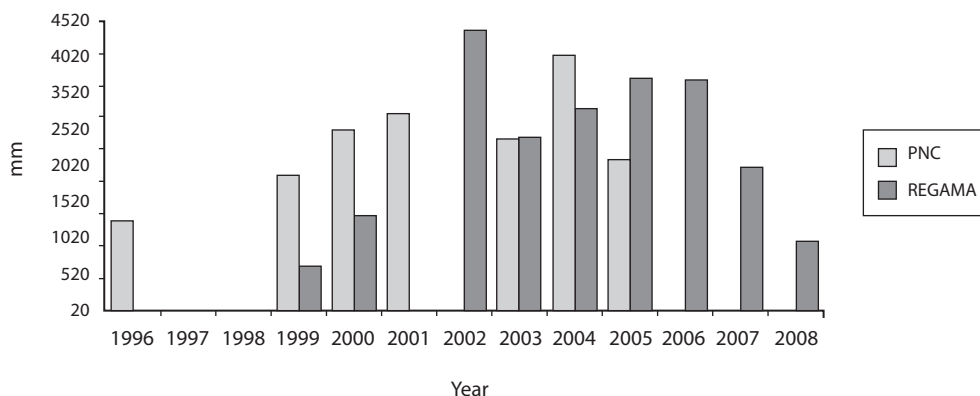
Fig. 4. Annual rainfall at PNC and REGAMA, 1996 to 2008.
