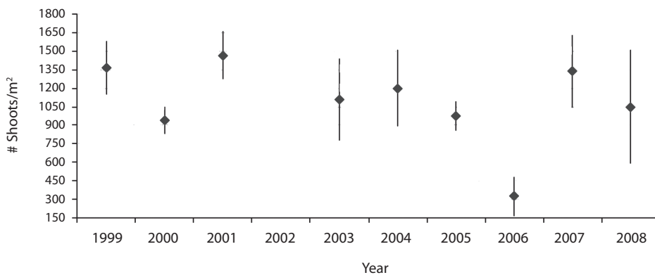
Fig. 14. Density ( \pm standard deviation) of Thalassia testudinum at Perezoso (PNC), 1999 to 2008.
