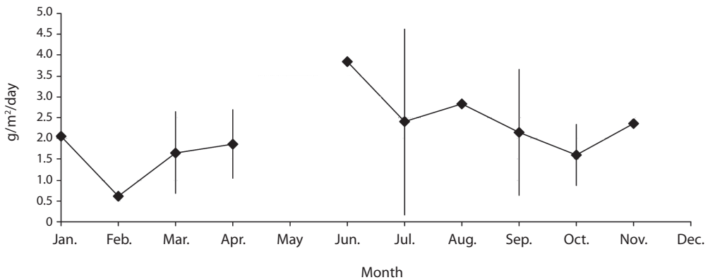
Fig. 11. Monthly average (1999-2009) of Thalassia testudinum productivity at Perezoso (PNC).
