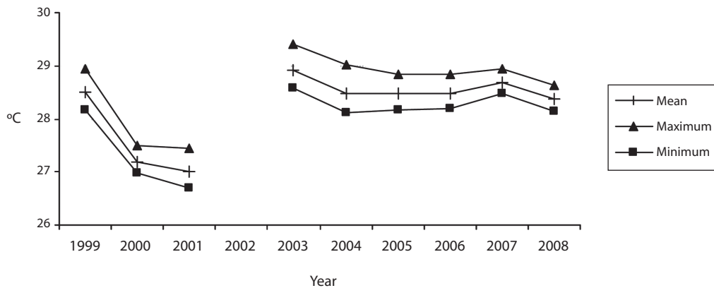
Fig. 5. Water temperature at the bank reef of Meager Shoal (PNC), 7m deep, from 1999 to 2008.
