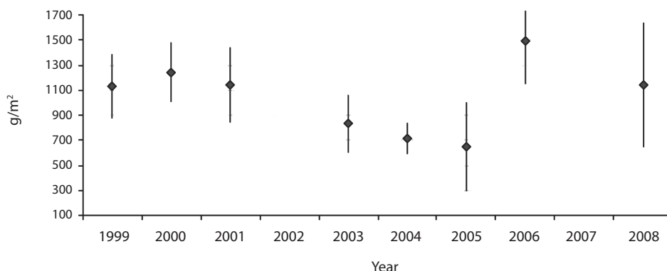
Fig. 15. Biomass ( \pm standard deviation, n=4 ) of Thalassia testudinum at Perezoso (PNC), 1999 to 2008.
