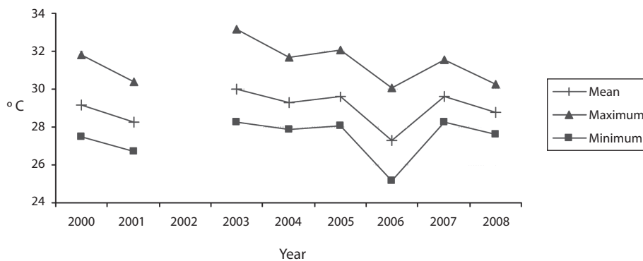
Fig. 6. Water temperature at the seagrass bed of Peresozo (PNC), 1.5m deep, from 2000 to 2008.
