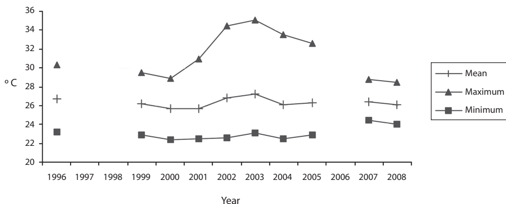
Fig. 2. Air temperature at Puerto Vargas, Parque Nacional Cahuita (PNC), 1996 to 2008.
