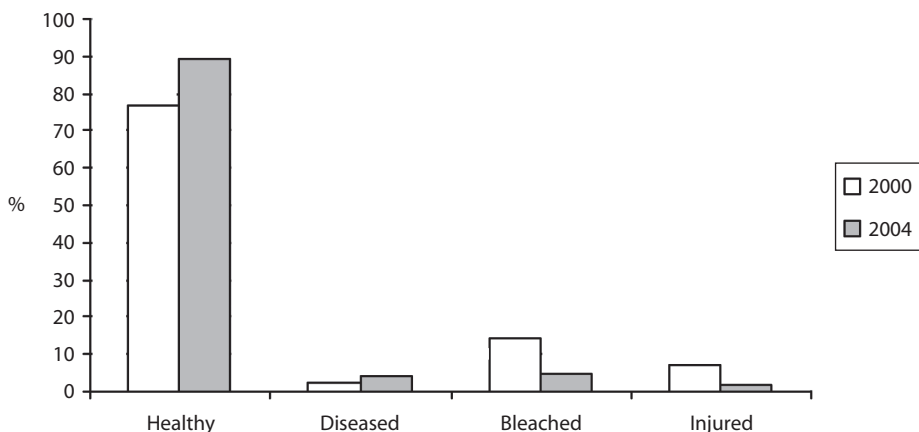
Fig. 9. General condition of coral colonies at Meager Shoal (PNC) in 2000 and 2004.
