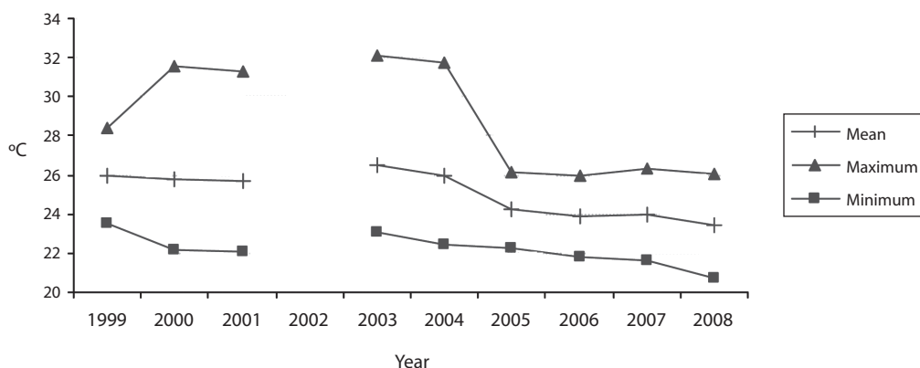
Fig. 3. Air temperature at Gandoca, Refugio Nacional de Vida Silvestre Gandoca-Manzanillo (REGAMA), 1999 to 2008.
