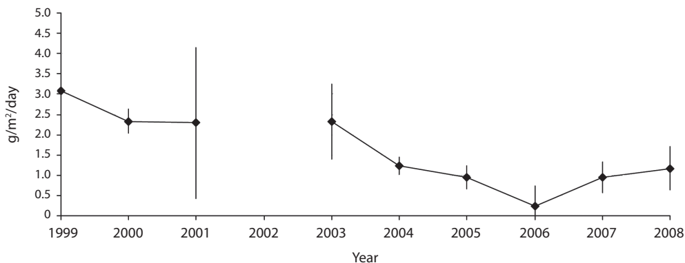
Fig. 12. Productivity ( \pm standard deviation) of Thalassia testudinum at Perezoso (PNC), 1999 to 2008.
