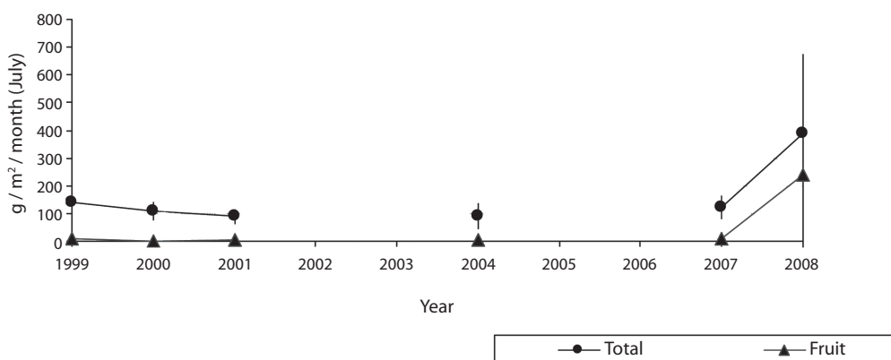
Fig. 16. Mangrove ( Rhizophora mangle ) mean ( \pm standard deviation) productivity in July at Gandoca (REGAMA), 1999 to 2008.
