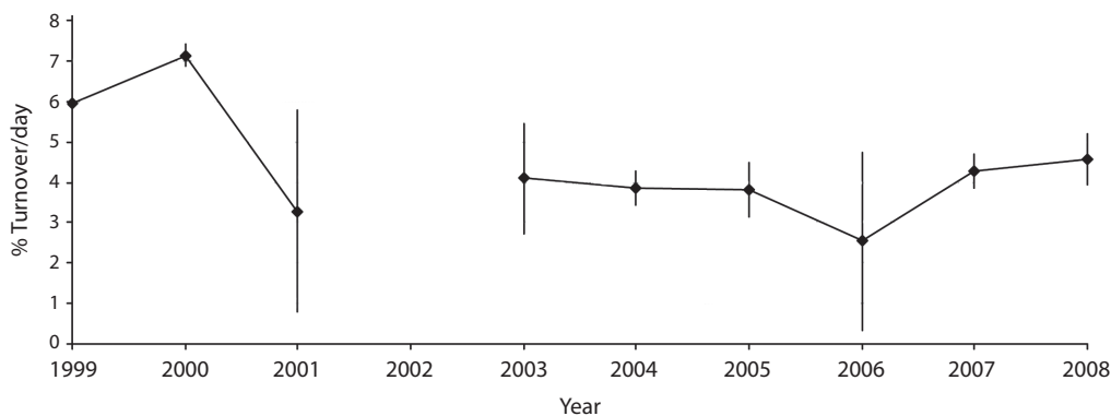
Fig. 13. Turnover rate ( \pm standard deviation) of Thalassia testudinum at Perezoso (PNC), 1999 to 2008.
