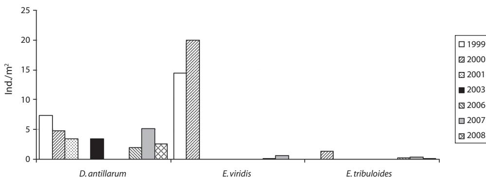
Fig. 10. Density (individuals/m 2 ) of the sea urchins, Diadema antillarum , Echinometra viridis and Eucidaris tribuloides at Meager Shoal (PNC), 1999 to 2008.
