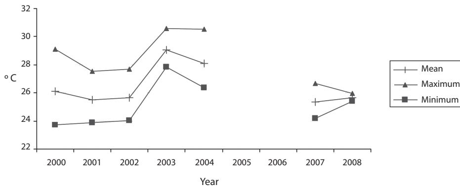
Fig. 7. Water temperature at the mangrove of Gandoca (REGAMA), 0.5m deep, from 2000 to 2008.
